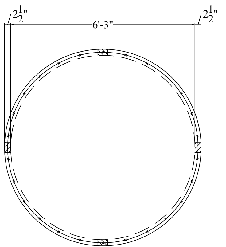
Plan View (Top Not Shown)
