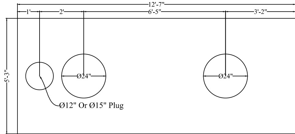
Top Slab Plan View
