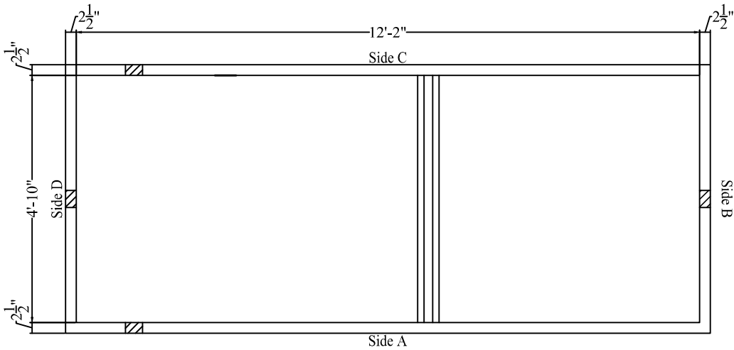
Plan View (Top Not Shown)
