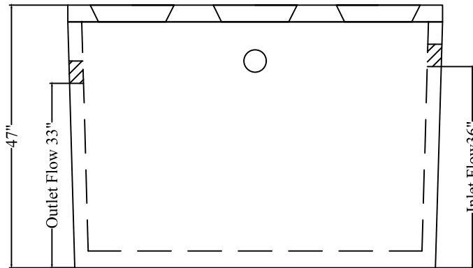
Layout Elevation
