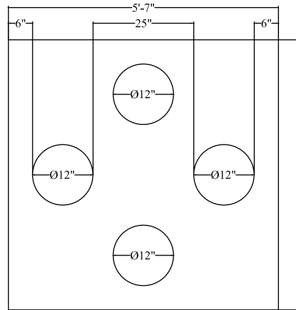
Top Slab Plan View
