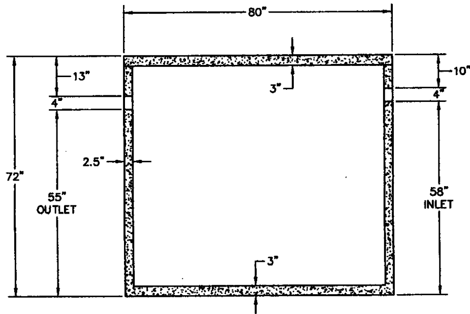
Section View
