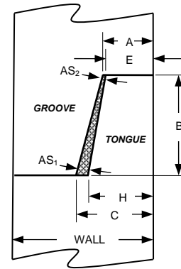
TONGUE & GROOVE JOINT
